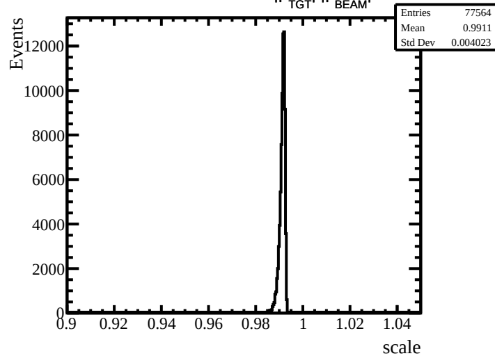
Momentum scale |\mathbf{p}_{\text{TGT}}|/|\mathbf{p}_{\text{BEAM}}|
