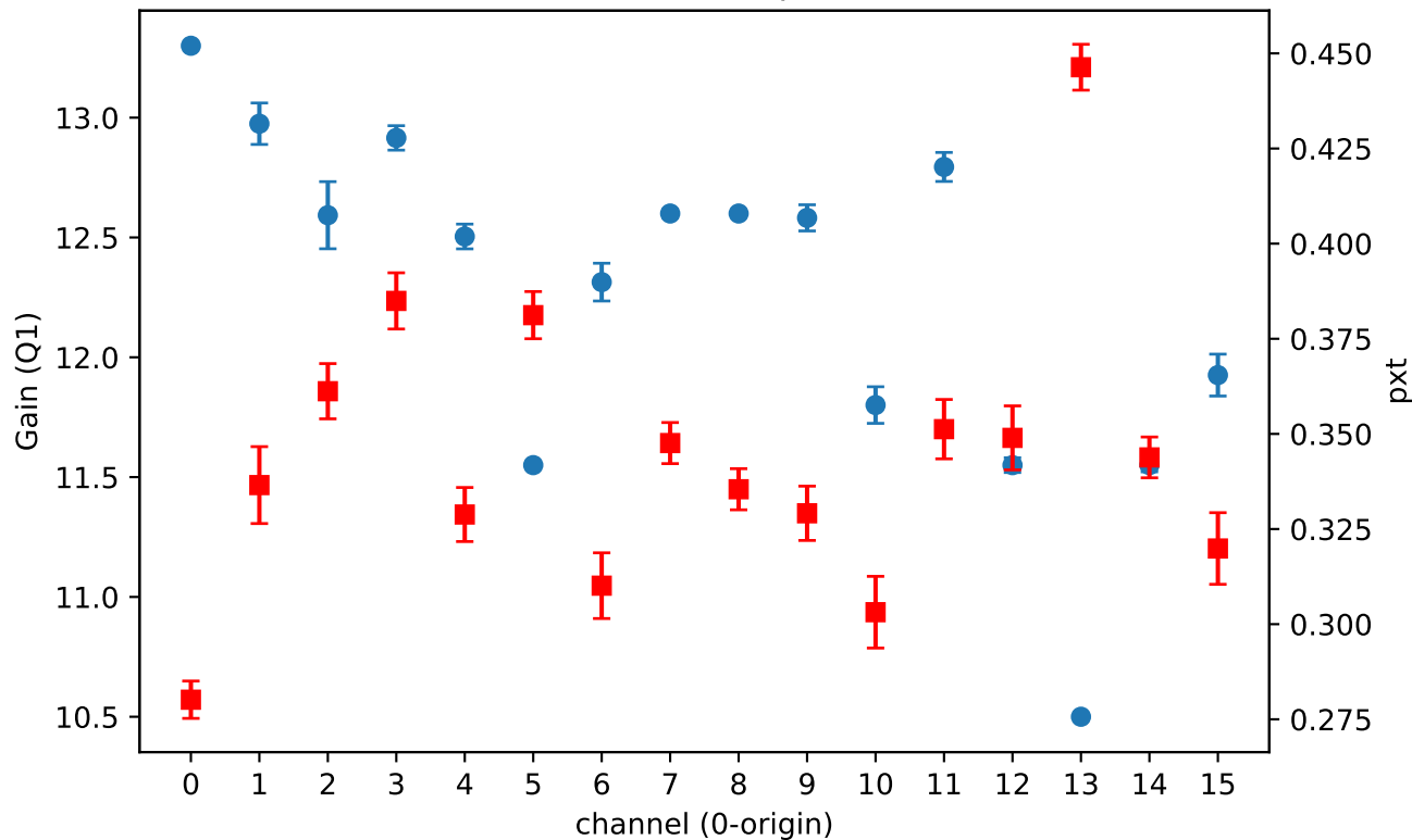
Board 3: Gain(Q1) and pxt vs channel
