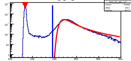
hist_t0_adc_u2
