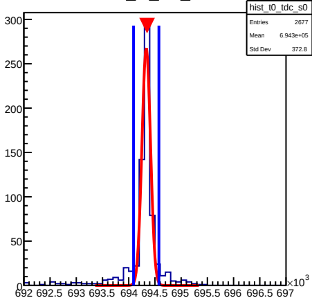
hist_t0_tdc_s0
