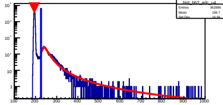
hist_bh2_adc_u4
