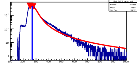
hist_bh2_adc_u5
