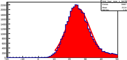
hist_bac_npe_s_bh28
