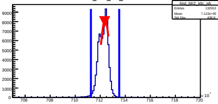
hist_bh2_tdc_s6
