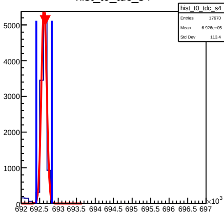
hist_t0_tdc_s4
