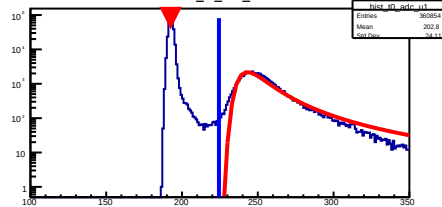
hist_t0_adc_u1
