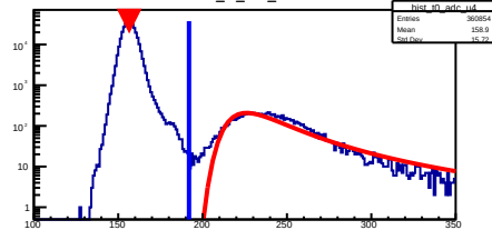
hist_t0_adc_u4
