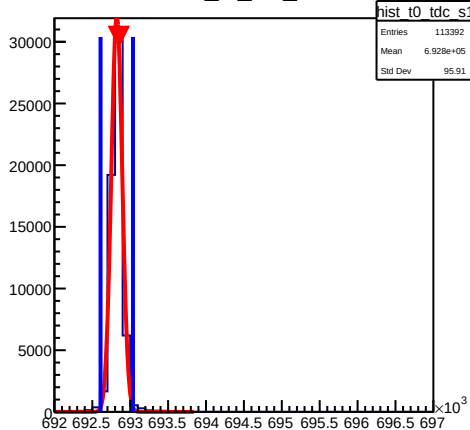
hist_t0_tdc_s1
