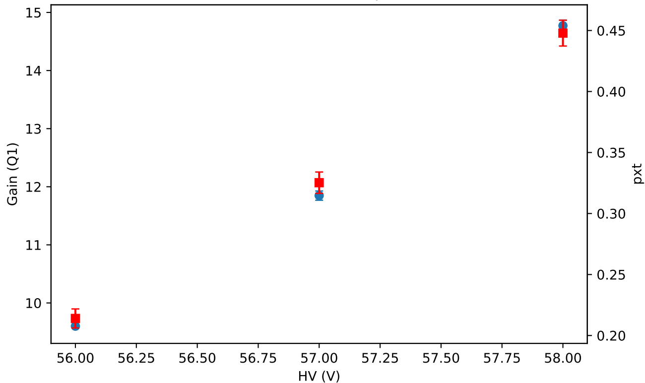
Board 0, ch=1: Q1 and pxt vs HV
