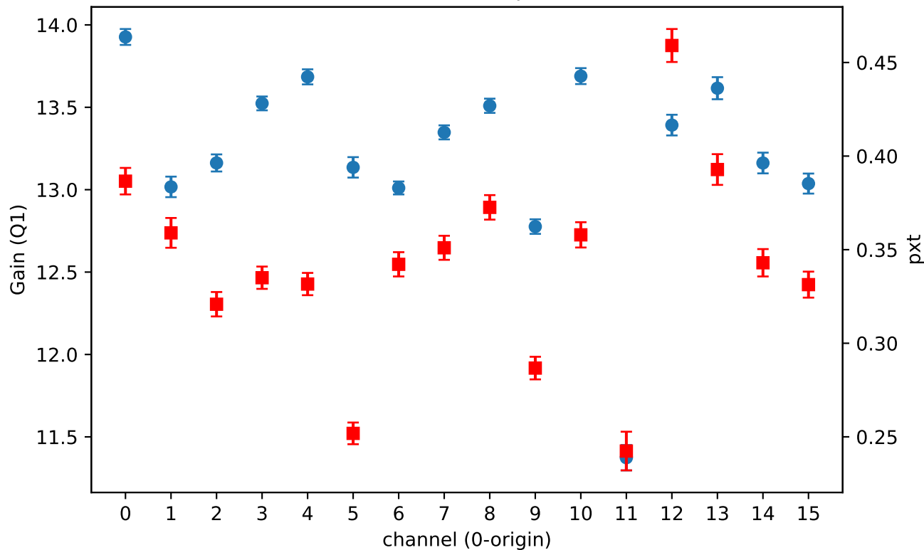
Board 2: Gain(Q1) and pxt vs channel
