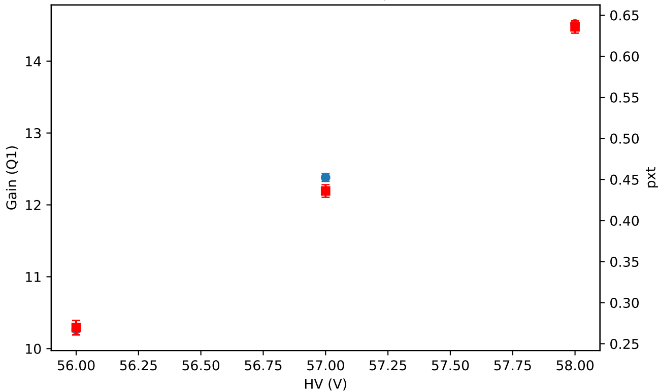
Board 1, ch=1: Q1 and pxt vs HV
