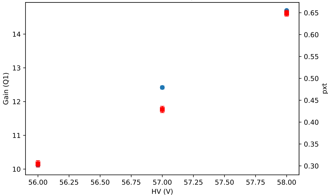
Board 2, ch=1: Q1 and pxt vs HV
