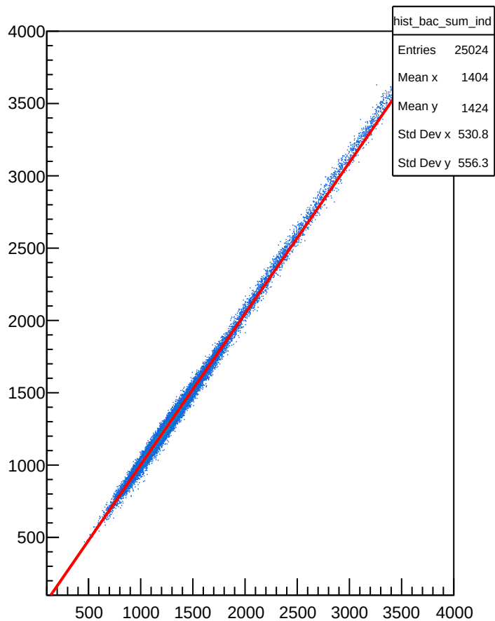
hist_bac_sum_ind
