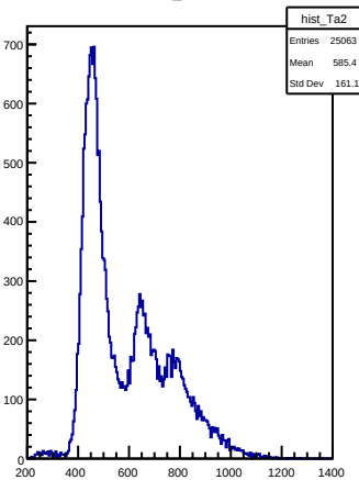
hist-Ta2
