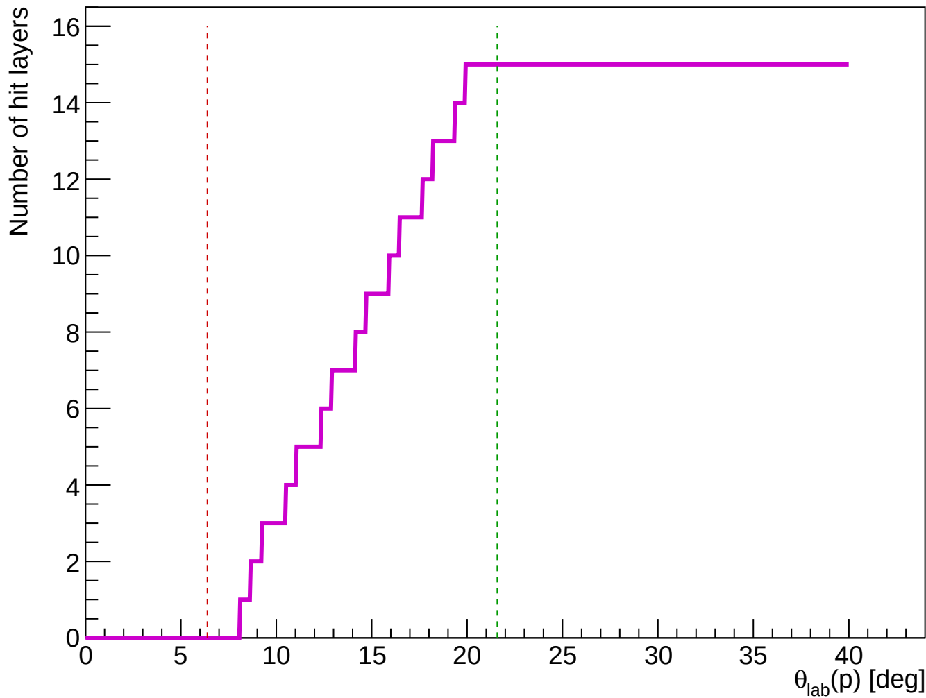
Number of CDC layers crossed by forward proton
