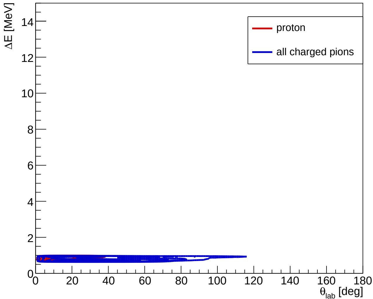
proton vs all charged pions in 10 mm plastic scintillator
