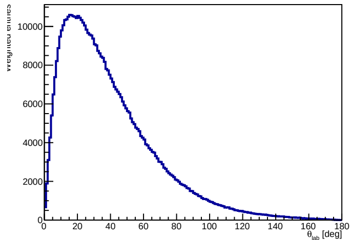
pions_all
