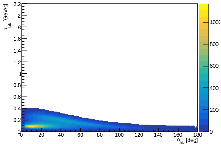
pions_all
