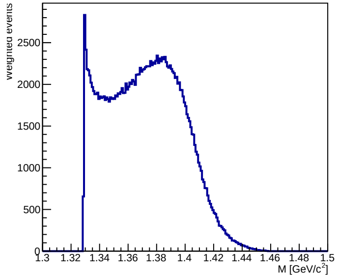
Sampled M(\Lambda(1405))
