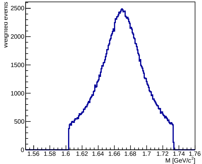
Sampled M(\Sigma(1670))
