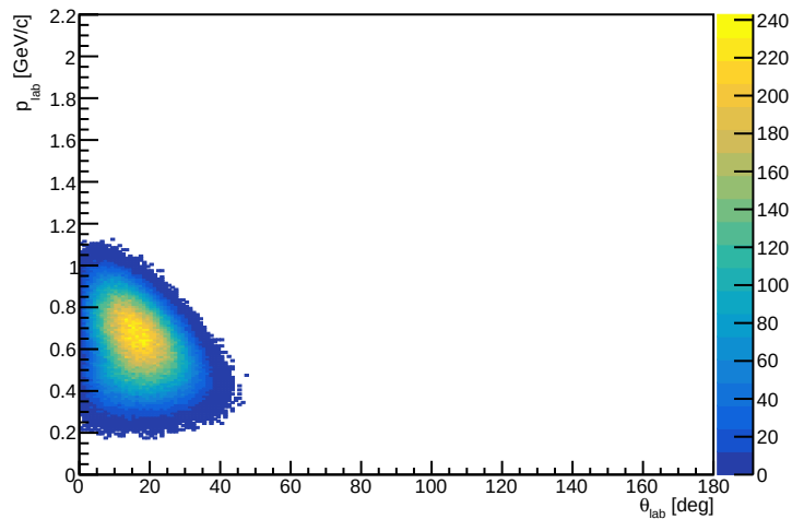
proton p vs \theta
