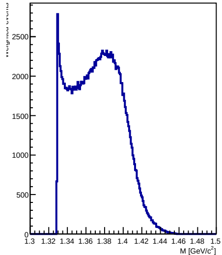
Reaction2 sampled M(\Lambda(1405))
