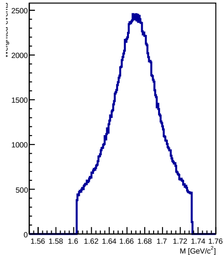
Reaction2 sampled M(\Sigma(1670))
