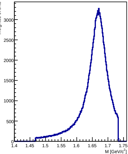
Reaction1 sampled M(\Sigma(1670))
