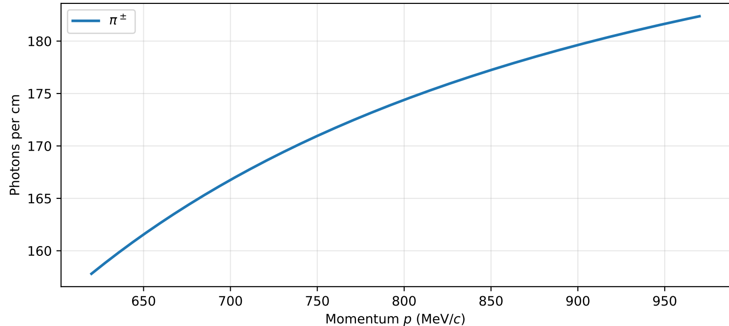
Frank-Tamm yield ( n = 1.115 , \lambda = 300\text{-}900\text{ nm} , z = 1 )
