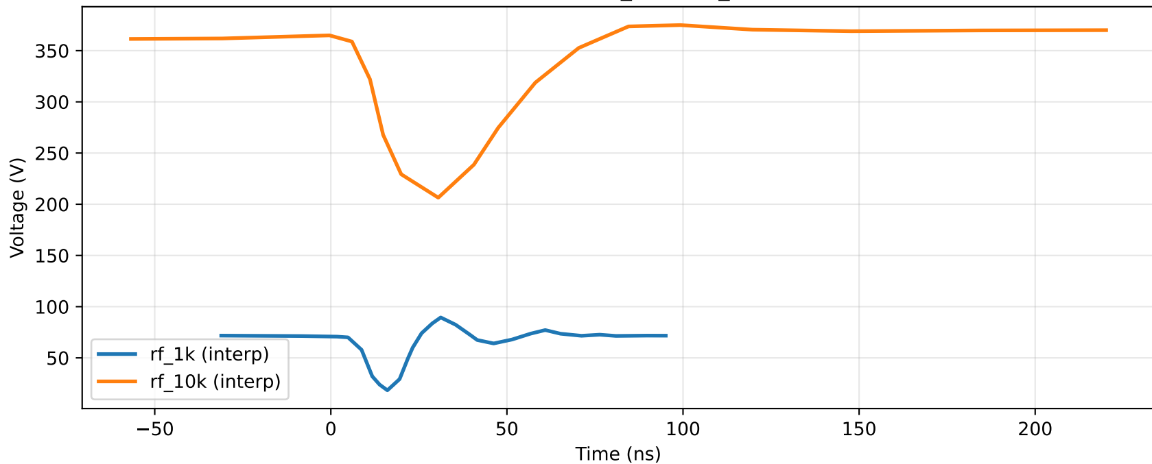
Waveforms: rf_1k vs rk_10k
