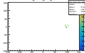
hist_bcout_bh2_2d14
