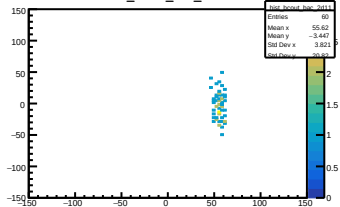
hist_bcout_bac_2d11
