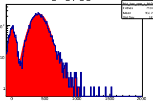
hist_bac_npe_s_bh26
