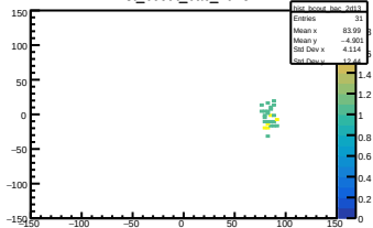
hist_bcout_bac_2d13
