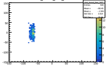
hist_bcout_bac_2d2
