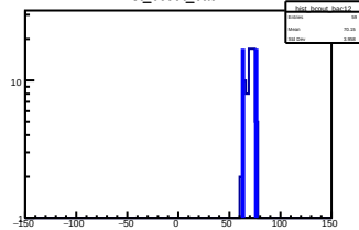
hist_bcount_bac12
