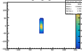
hist_bcout_bh2_2d7
