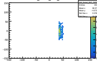
hist_bcout_bh2_2d10
