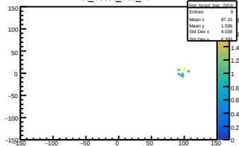
hist_bcout_bac_2d14
