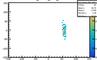
hist_bcout_bh2_2d11
