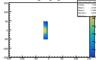
hist_bcout_bh2_2d6
