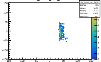
hist_bcout_bac_2d10
