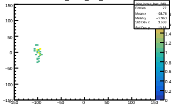
hist_bcout_bac_2d0
