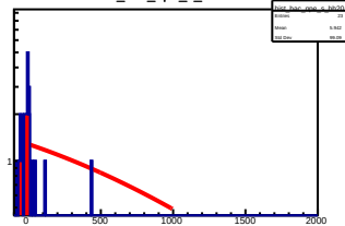
hist_bac_npe_s_bh20
