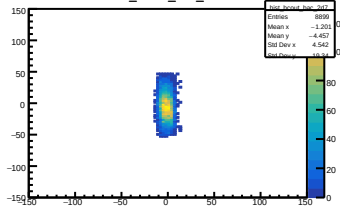
hist_bcout_bac_2d7
