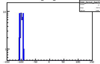
hist_bcount_bac0
