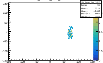
hist_bcout_bac_2d12
