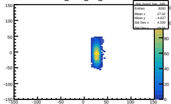
hist_bcout_bac_2d9
