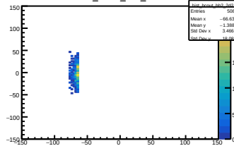
hist_bcout_bh2_2d2
