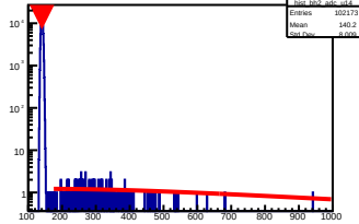
hist_bh2_adc_u14
