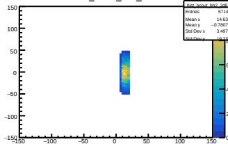
hist_bcout_bh2_2d8
