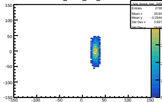
hist_bcout_bac_2d9
