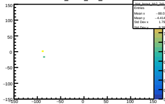
hist_bcout_bh2_2d1
