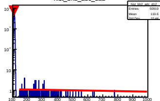
hist_bh2_adc_d12
