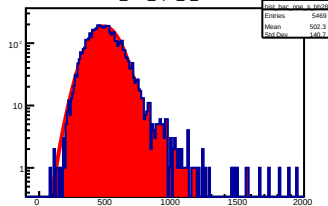
hist_bac_npe_s_bh28
