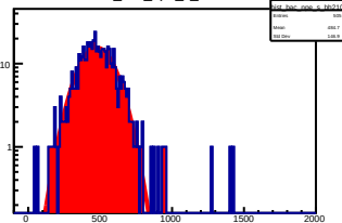
hist_bac_npe_s_bh210
