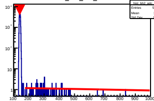
hist_bh2_adc_u14
