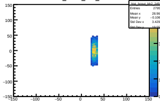
hist_bcout_bh2_2d9
