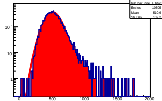
hist_bac_npe_s_bh26
