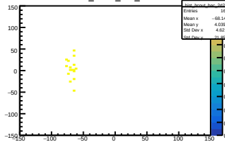
hist_bcout_bac_2d2
