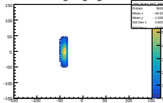
hist_bcout_bh2_2d4
