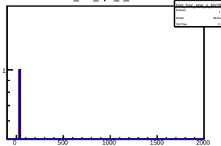
hist_bac_npe_s_bh20
