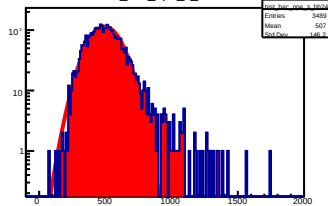
hist_bac_npe_s_bh24
