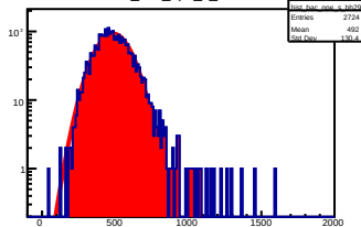
hist_bac_npe_s_bh29
