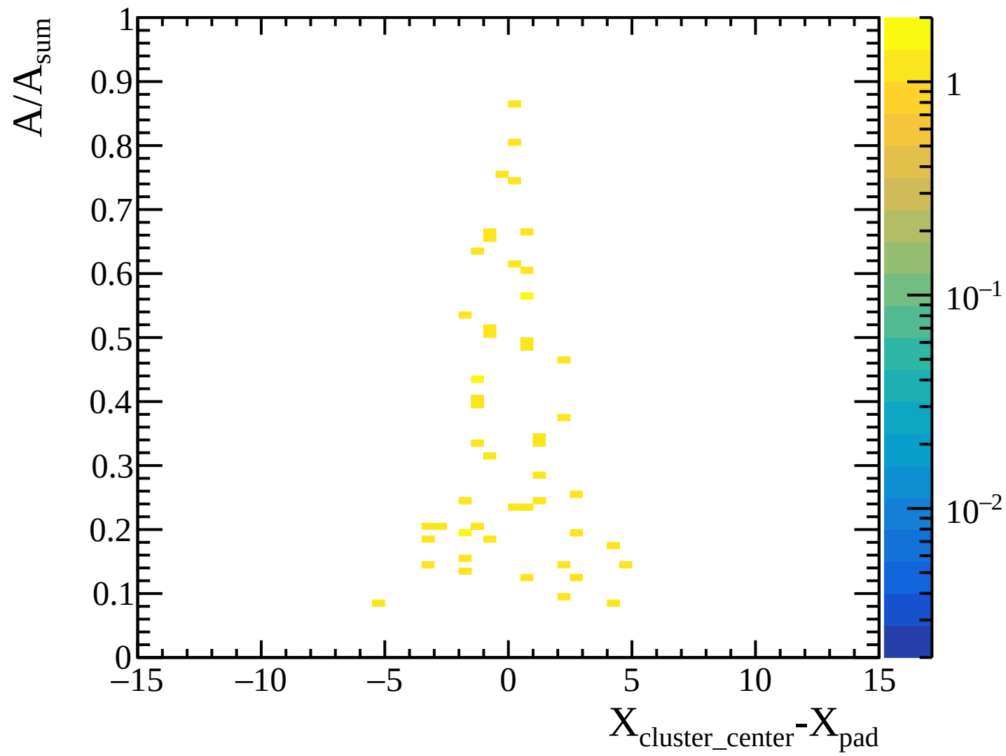
TPC transverse diffusion: layer 00 [Transverse_Diffusion_Layer00]
