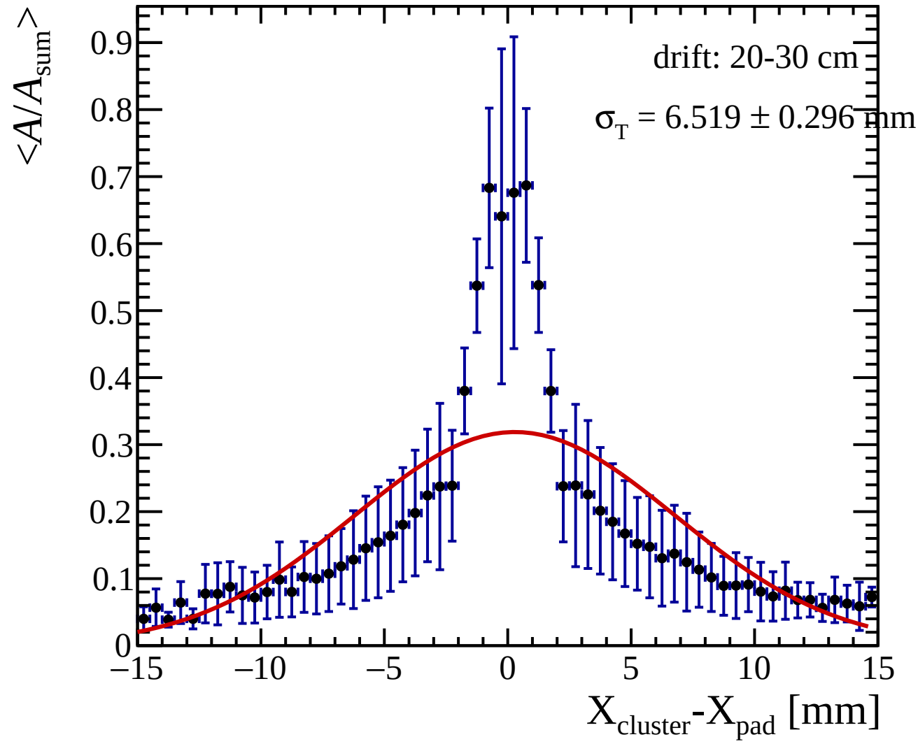
Transverse-diffusion profile: Drift distance = 20-30 cm
