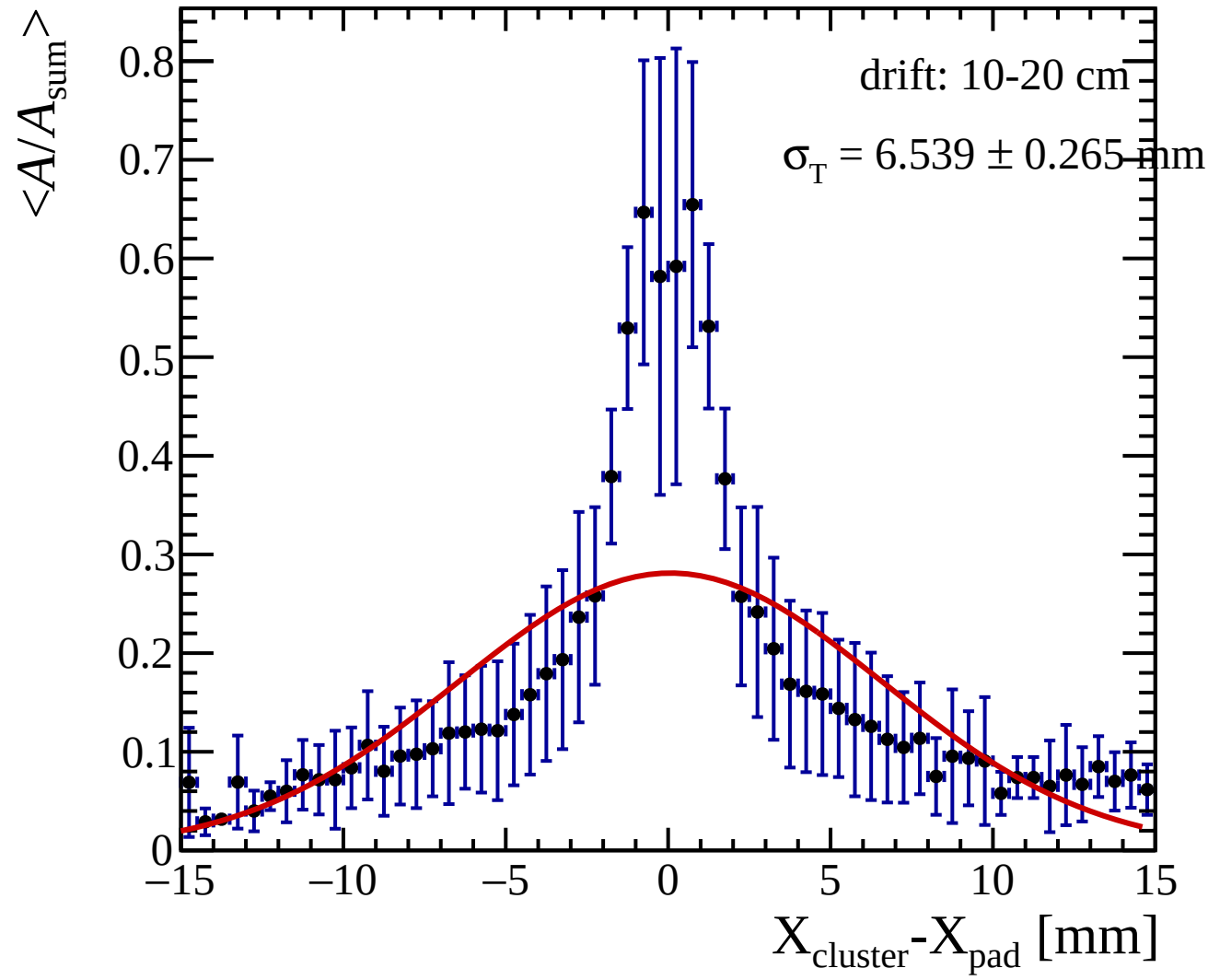
Transverse-diffusion profile: Drift distance = 10-20 cm
