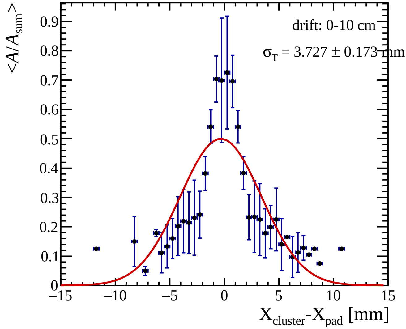
Transverse-diffusion profile: Drift distance = 0-10 cm
