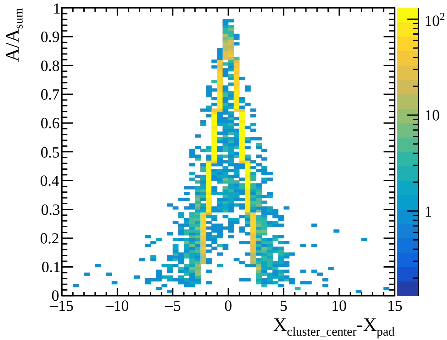
TPC transverse diffusion: layer 21 [Transverse_Diffusion_Layer21]
