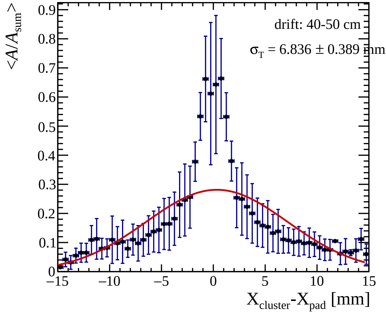
Transverse-diffusion profile: Drift distance = 40-50 cm
