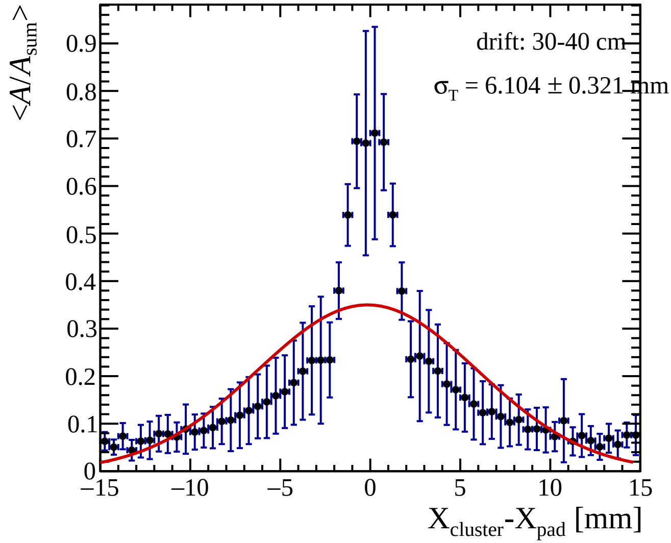
Transverse-diffusion profile: Drift distance = 30-40 cm
