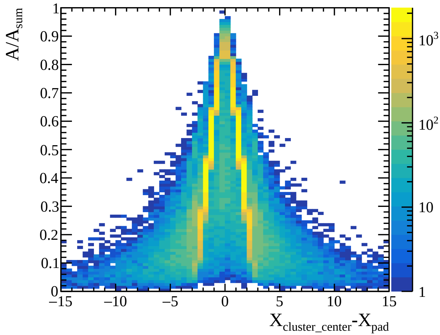
TPC transverse diffusion: all layers [Transverse_Diffusion]
