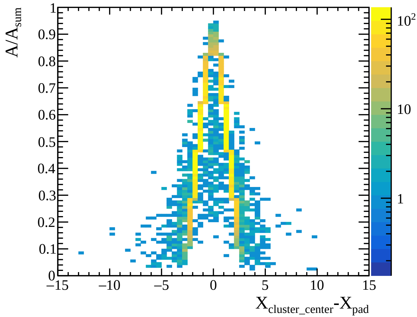
TPC transverse diffusion: layer 22 [Transverse_Diffusion_Layer22]
