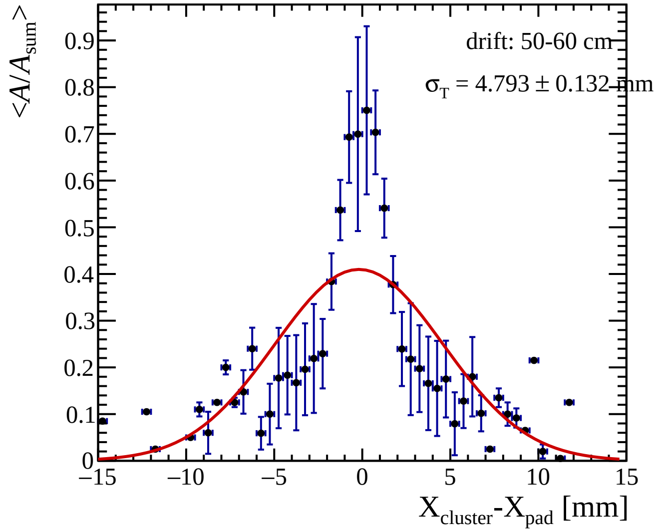
Transverse-diffusion profile: Drift distance = 50-60 cm
