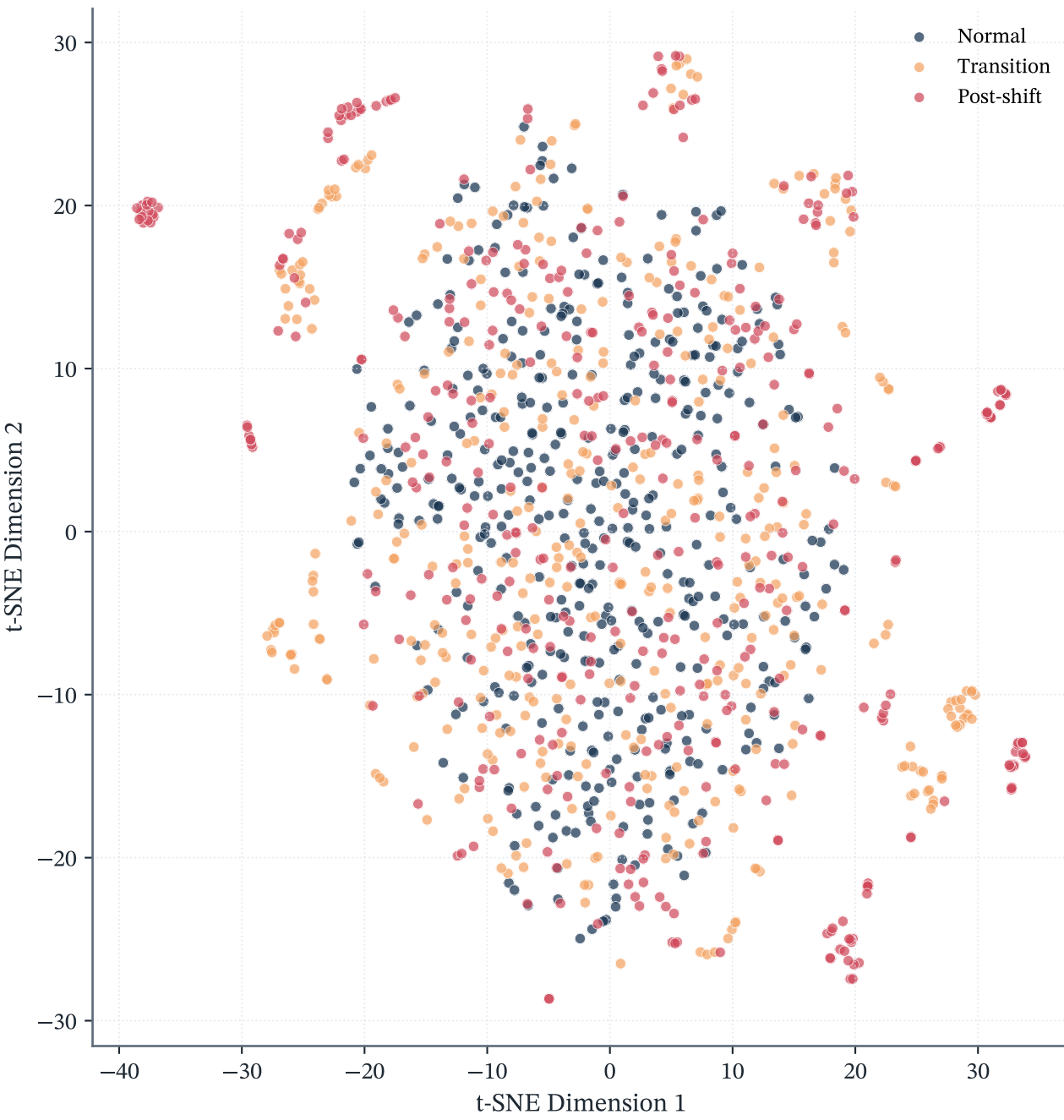
t-SNE View of the TEP Dataset under Temporal Shift
