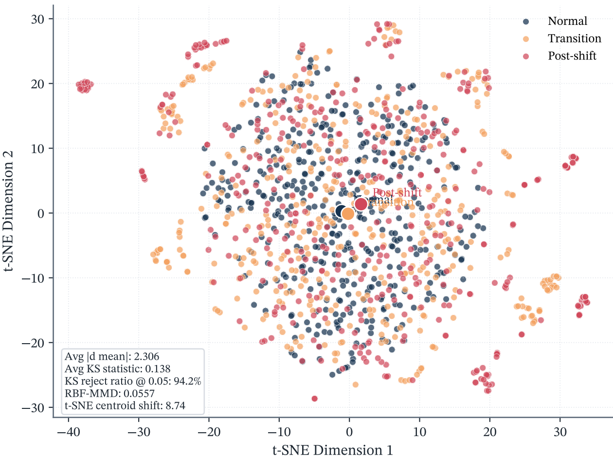
Figure E1(a). t-SNE View of the TEP Dataset under Temporal Shift
