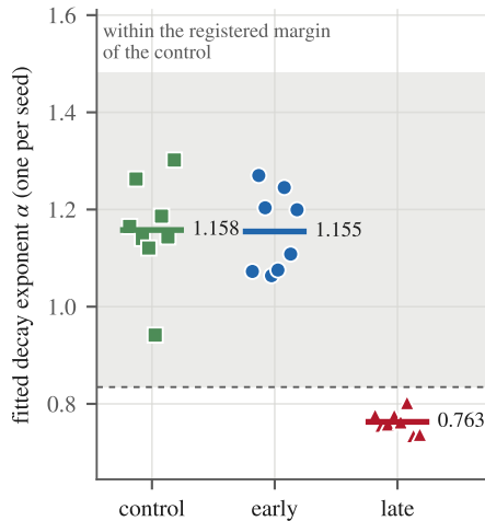
(b) every seed, not one outlier
