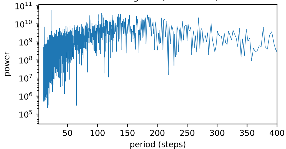
Periodogram (detrended)
