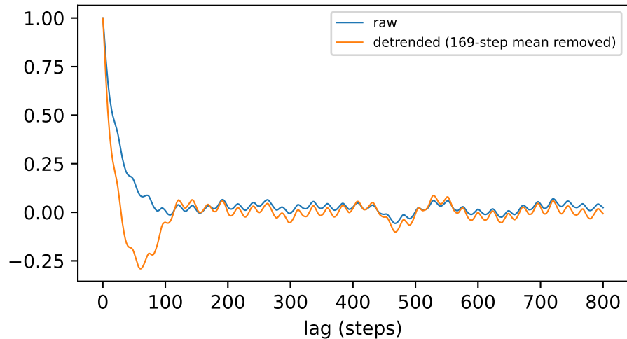
Training-split ACF
