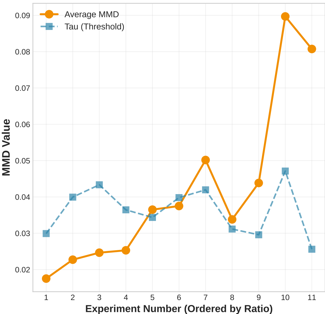
Average MMD vs Sample Ratio
