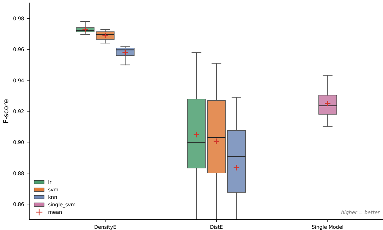
F-score distributions across ensemble methods and base learners
