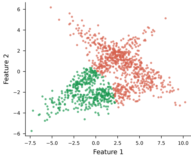
a K-means (ARI = 0.23)
