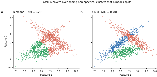
Fig. 7. Cluster assignments on three elongated, overlapping Gaussian components ( K = 3 given to both algorithms). (a) K-means fragments the components along axis-aligned boundaries ( \text{ARI} = 0.23 ); (b) the Gaussian mixture recovers the underlying structure ( \text{ARI} = 0.70 ). Colours denote recovered cluster membership matched to the ground-truth components.
