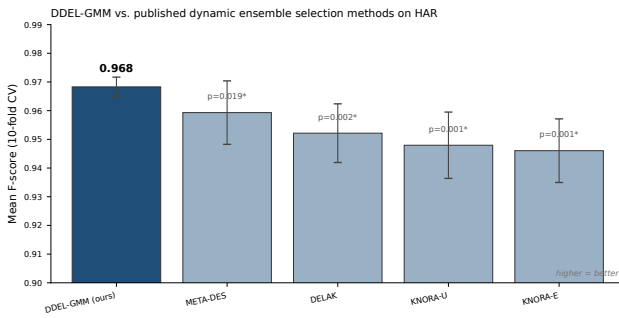
Fig. 6. Mean F-score of DDEL-GMM against published dynamic ensemble selection methods on the HAR dataset. Error bars are \pm 1 standard deviation over the 10 cross-validation folds; annotations report the one-sided Wilcoxon signed-rank p -value of DDEL-GMM against each baseline ( *p < 0.05 ).
