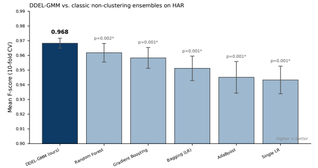
Fig. 8. Mean F-score of DDEL-GMM against classic non-clustering ensemble methods on the HAR dataset. Error bars are \pm 1 standard deviation over the 10 cross-validation folds; annotations report the one-sided Wilcoxon signed-rank p -value of DDEL-GMM against each baseline ( *p < 0.05 ).
