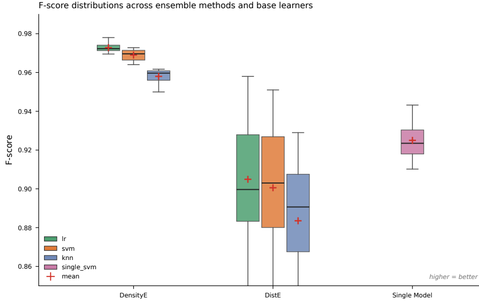
Fig. 5. Comparison of F-score Distributions Across Different Ensemble Methods and Base Learners
