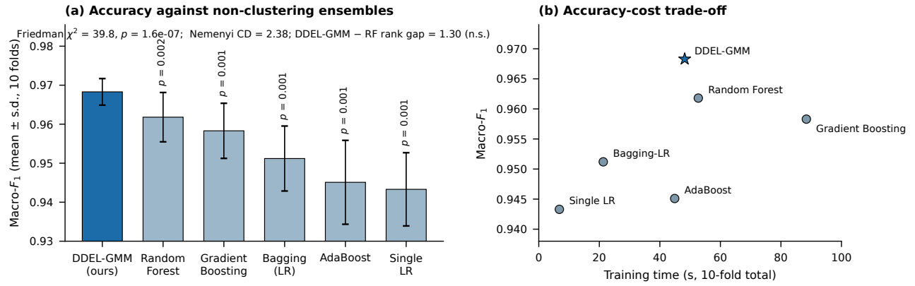
Fig. 8. DDEL-GMM against classic non-clustering ensemble methods on the HAR dataset. (a) Mean macro- F_1 with error bars of \pm 1 standard deviation over the 10 cross-validation folds; annotations give the one-sided Wilcoxon signed-rank p -value against each baseline, and the header reports the Friedman omnibus test and the Nemenyi critical difference. The DDEL-GMM–random-forest rank gap falls below that critical difference and is marked not significant. (b) Accuracy–cost trade-off: mean macro- F_1 against total 10-fold training time.
