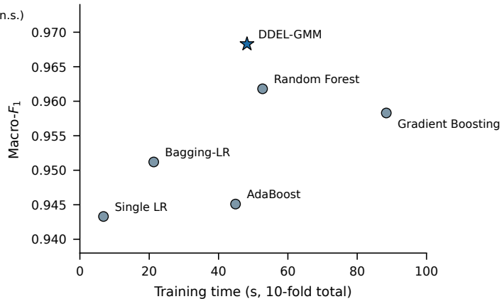
(b) Accuracy-cost trade-off
