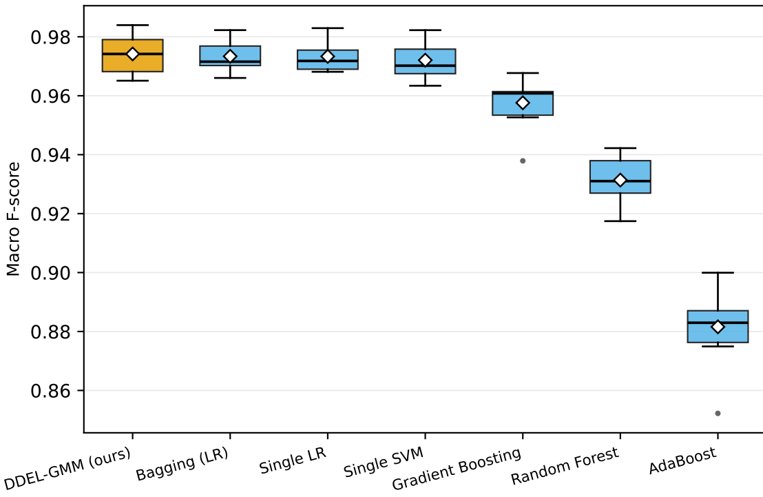
DDEL-GMM vs non-clustering baselines
