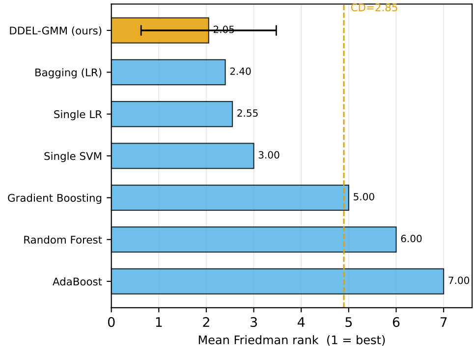
DDEL-GMM vs non-clustering baselines
