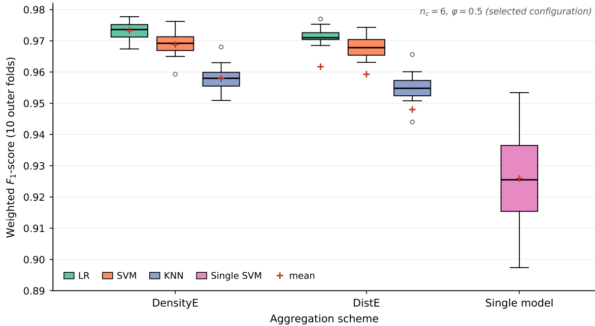
Fig. 4. Per-fold distribution of the weighted F_1 -score over the ten outer cross-validation folds at the selected configuration ( n_c = 6 , \varphi = 0.5 ), for the density-weighted (DensityE) and distance-weighted (DistE) aggregation schemes with each base learner, together with the single-SVM reference. Boxes span the interquartile range, the horizontal rule is the median, red crosses mark the mean, and circles are folds beyond 1.5 \times \text{IQR} . The two clustering-based schemes overlap for every base learner, but DensityE is markedly more concentrated: its interquartile ranges are narrower and it produces no low-side outlier folds. The decision-tree learner is omitted; its scores lie near 0.82 and fall outside the plotted range (see Table 1).
