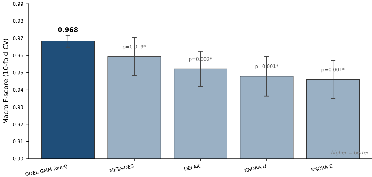
DDEL-GMM vs. published dynamic ensemble selection methods on HAR
