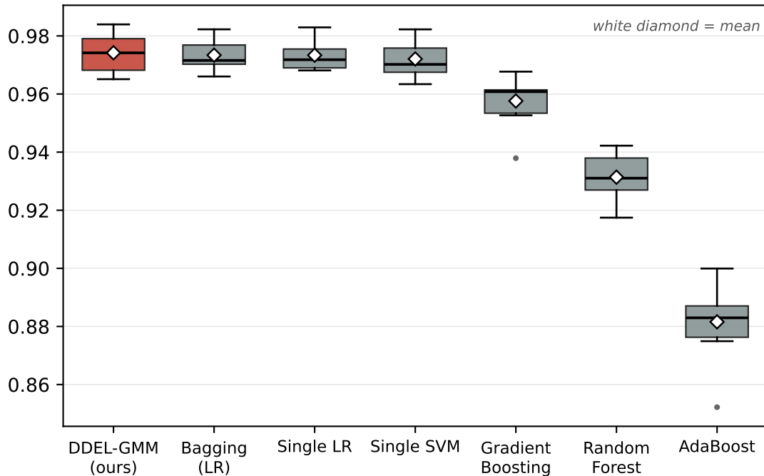
(a) Per-fold F-score, 10-fold stratified CV
