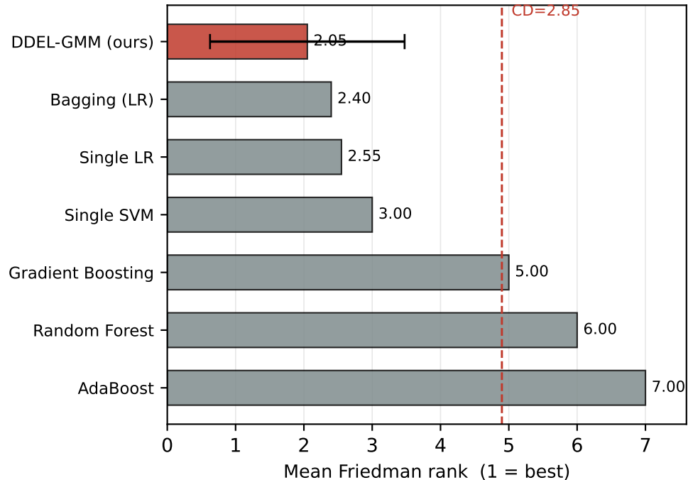
(b) Mean rank and Nemenyi critical difference
