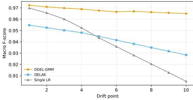
Fig. 11. Macro F-score trajectories across ten simulated concept-drift windows for DDEL-GMM, DELAK, and a single logistic-regression classifier. DDEL-GMM degrades 3.6\times less than DELAK and 8.7\times less than the single learner, confirming that the density-based weighting maintains effective competence estimates as the data distribution shifts.
