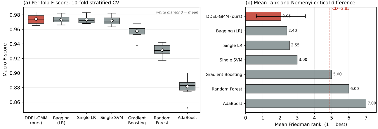
Fig. 10. DDEL-GMM against classic non-clustering ensemble methods on the HAR dataset, from measured per-fold results. (a) Distribution of macro F-scores over the 10 stratified cross-validation folds; the white diamond marks the mean. The four leftmost methods overlap substantially. (b) Mean Friedman rank with the Nemenyi critical difference at \alpha = 0.05 ( CD = 2.85 , k = 7 , N = 10 ); the dashed line marks the threshold beyond which a baseline is separated from DDEL-GMM. Gradient boosting, random forests, and AdaBoost fall beyond it; bagging, the single logistic-regression model, and the support vector machine do not.
