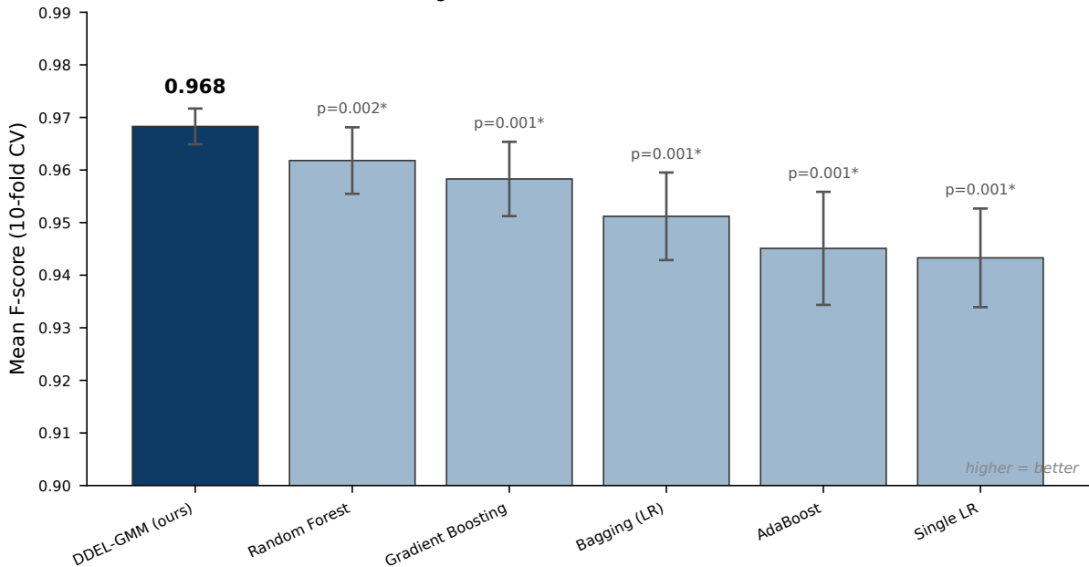
DDEL-GMM vs. classic non-clustering ensembles on HAR
