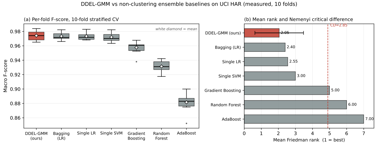
Fig. 8. DDEL-GMM against classic non-clustering ensemble methods on the HAR dataset, from measured per-fold results. (a) Distribution of macro F-scores over the 10 stratified cross-validation folds; the white diamond marks the mean. The four leftmost methods overlap substantially. (b) Mean Friedman rank with the Nemenyi critical difference at \alpha = 0.05 ( CD = 2.85 , k = 7 , N = 10 ); the dashed line marks the threshold beyond which a baseline is separated from DDEL-GMM. Only random forests and AdaBoost fall beyond it.
