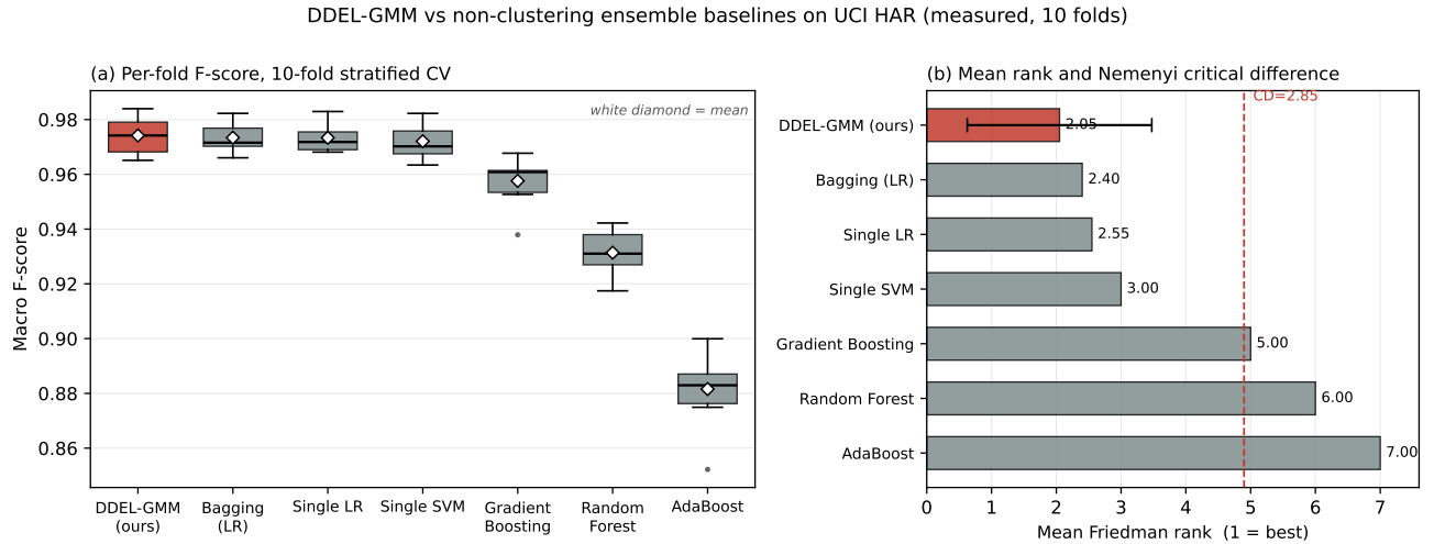
Fig. 9. DDEL-GMM against classic non-clustering ensemble methods on the HAR dataset, from measured per-fold results. (a) Distribution of macro F-scores over the 10 stratified cross-validation folds; the white diamond marks the mean. The four leftmost methods overlap substantially. (b) Mean Friedman rank with the Nemenyi critical difference at \alpha = 0.05 ( CD = 2.85 , k = 7 , N = 10 ); the dashed line marks the threshold beyond which a baseline is separated from DDEL-GMM. Gradient boosting, random forests, and AdaBoost fall beyond it; bagging, the single logistic-regression model, and the support vector machine do not.
