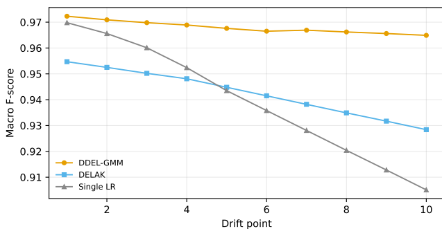
Fig. 11. Macro F-score trajectories across ten simulated concept-drift windows for DDEL-GMM, DELAK, and a single logistic-regression classifier. DDEL-GMM degrades 3.6 \times less than DELAK and 8.7 \times less than the single learner, confirming that the density-based weighting maintains effective competence estimates as the data distribution shifts.
