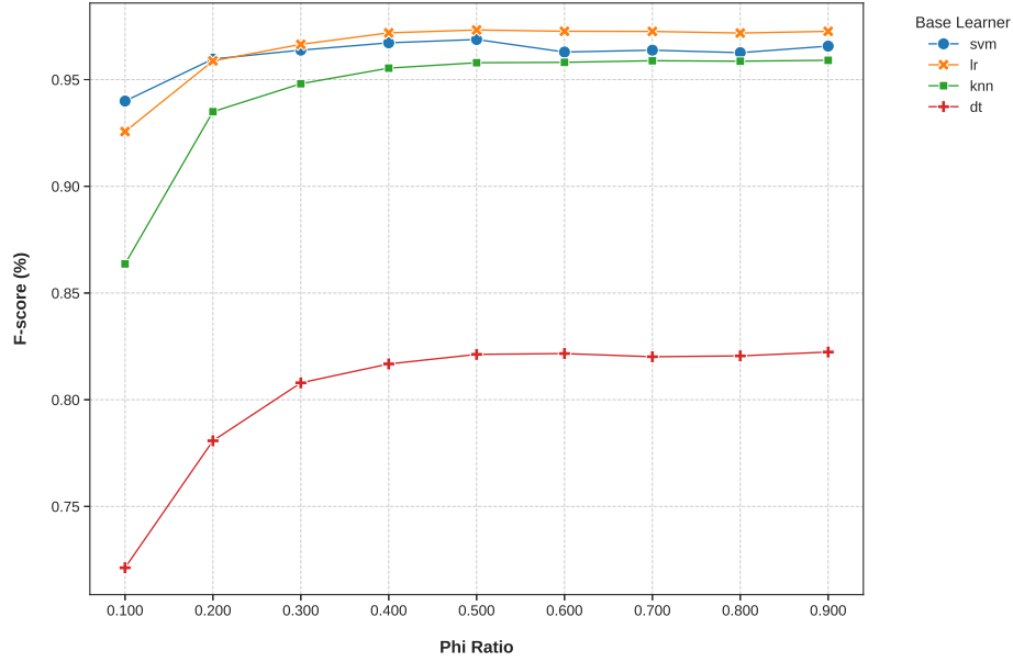
Fig. 3. F-score vs Sampling Ratio for Density ensemble method
