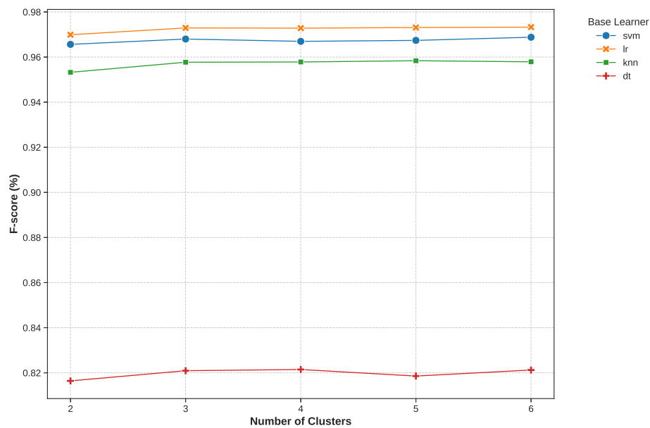
Fig. 4. F-score vs Number of Clusters for Density ensemble method
