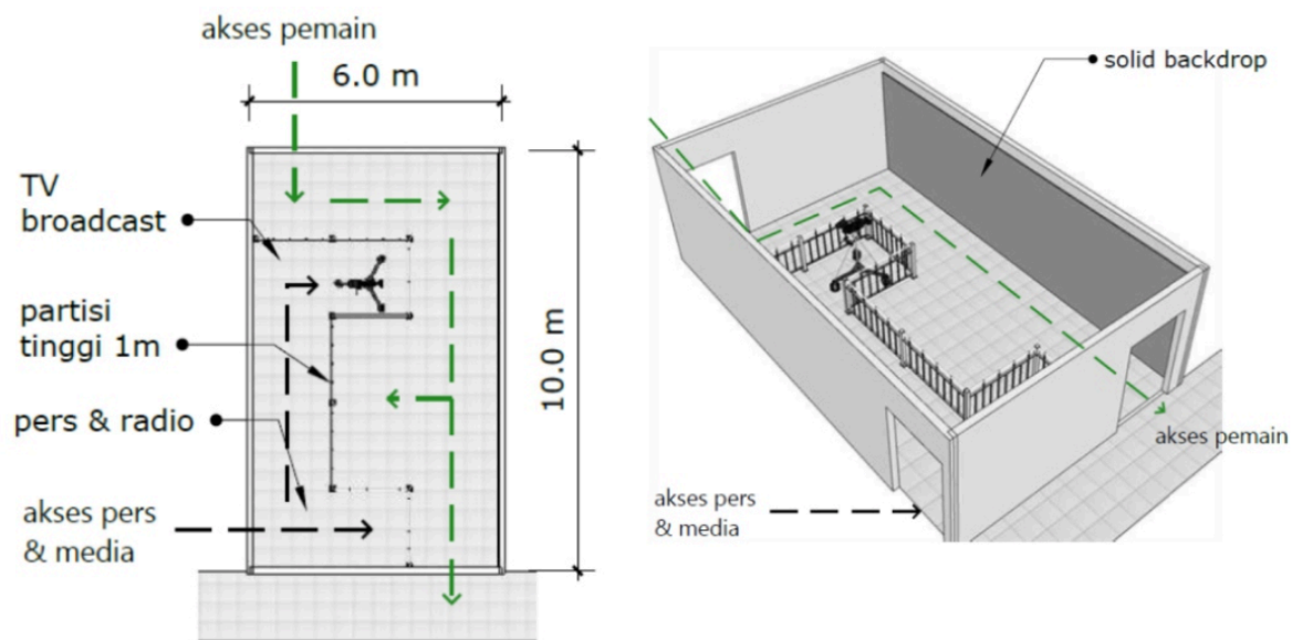
Gambar 3.3 Ilustrasi area mixed zone .
