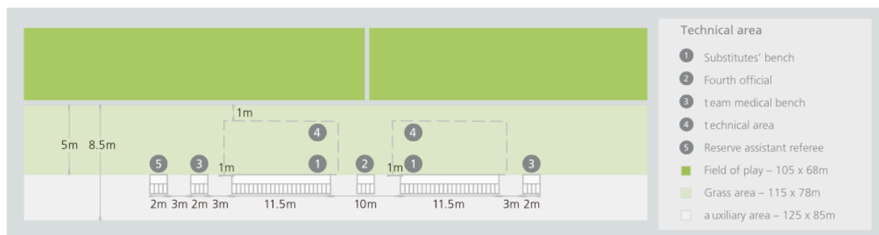
Gambar 2.4 Detail area teknik & bench.
