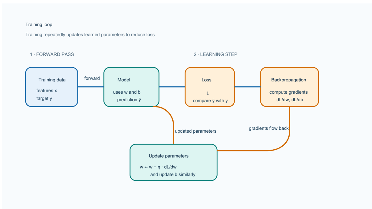
Figure 9. Training alternates a forward calculation with a learning step that uses error information to update parameters.
