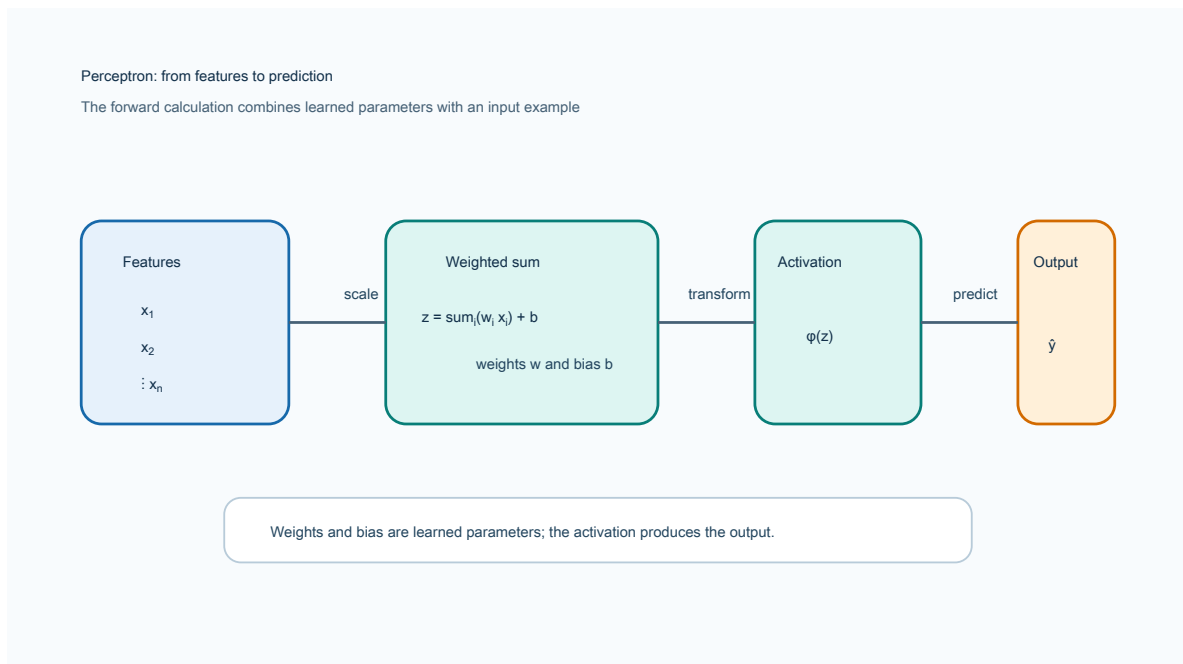
Figure 5. A perceptron scales features with weights, adds a bias, and passes the combined value through an activation function.
