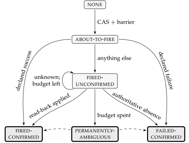
Fig. 1. The intent state machine, generated from the transition table in aep_core/core/intents.py . Solid edges are automated; the dashed edges from PERMANENTLY-AMBIGUOUS are the operator-only transitions. Every state with a thick border is terminal for automated reconciliation. There is no edge back into ABOUT-TO-FIRE — that absence is what “never silently re-dispatched” means, and it is enforced inside the atomic script rather than by the caller.
