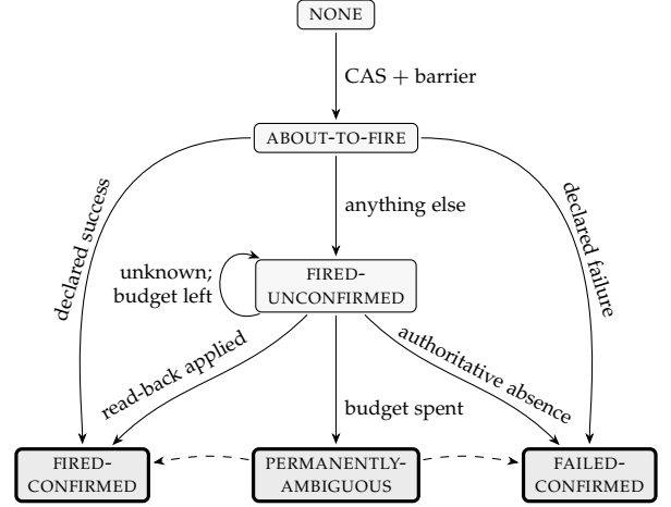
Fig. 1. The intent state machine, generated from the transition table in the implementation. Solid edges are automated; the dashed edges from PERMANENTLY-AMBIGUOUS are the operator-only transitions. Every state with a thick border is terminal for automated reconciliation. There is no edge back into ABOUT-TO-FIRE. That absence is what “never silently re-dispatched” means, and it is enforced inside the atomic script rather than by the caller.
