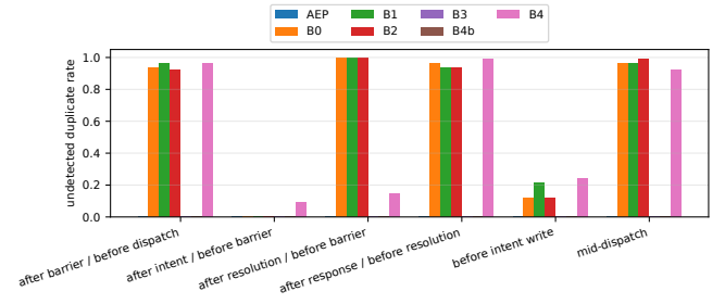
Fig. 2. Undetected duplicate rate by crash point, crashed regime, pooled over endpoint capabilities weighted by executions. The baselines' rate is near one wherever the kill lands once the request is on the wire, which is why a mechanism acting only after the call cannot help. At before_intent_write , where nothing has been sent, it falls back to the timeout background of Section 6.1.
