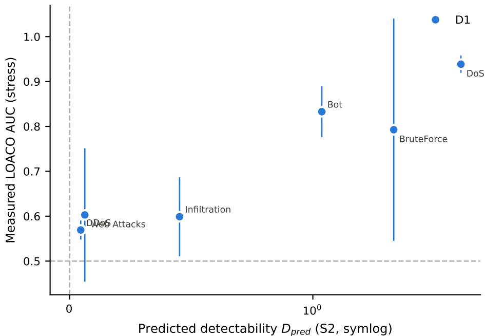
(a) D1 families Spearman \rho = 0.89 [0.45, 1.00], n = 6
