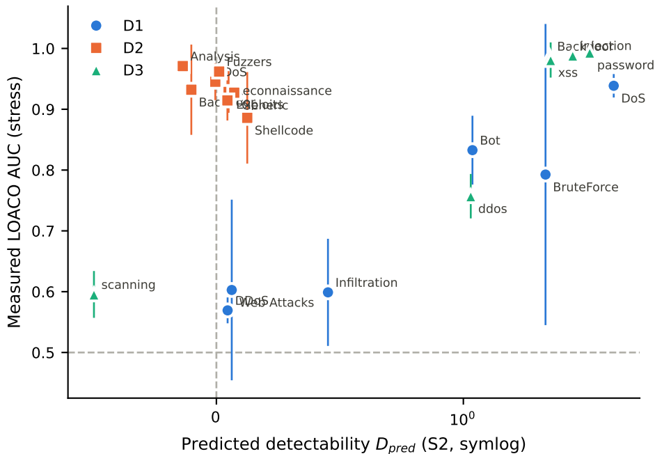
(b) pooled: D1 families + D2 + D3 (grouped_random) Spearman \rho = 0.33 [-0.25, 0.72], n = 20
